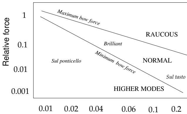
Fig. 4. The original Schelleng diagram, reproduced from [24].
