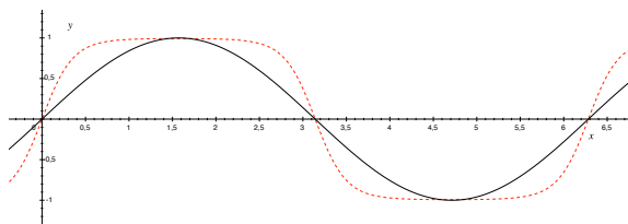
Figure 3: Sine wave (black) vs. distorted sine wave produced by f(x) = \tanh(\sin(x) * 2.8) (red, striped).
